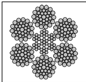
6x36WS
