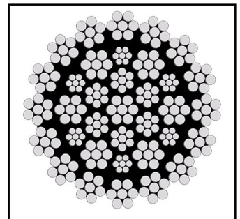
35x7
