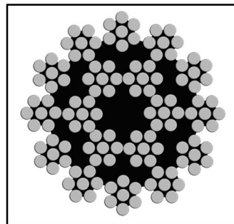
18x7
