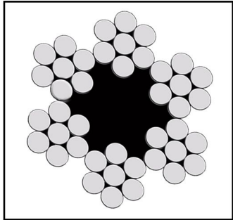
6x7
