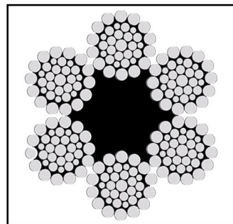
6x36WS+FC
